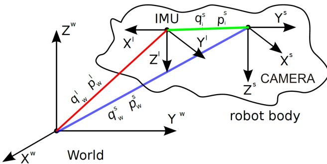
Fig. 8. Setup depicting the robot body with its sensors with respect to a world reference frame. The system state vector is X = \{p_w^i \ v_w^i \ q_w^i \ b_\omega \ b_a \ \lambda \ p_i^s \ q_i^s\} whereas p_w^s and q_w^s denote the robot's sensor measurements in (a possibly scaled) position and attitude respectively in a world frame.
