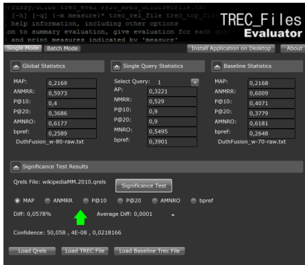
Figure 1: The TREC_Files Evaluator.
