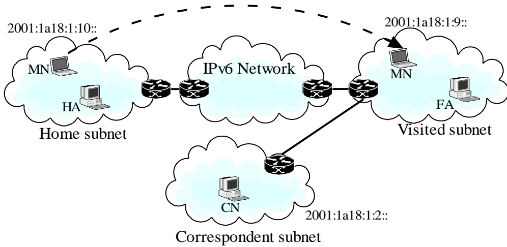
Fig. 2 Testbed Topology
