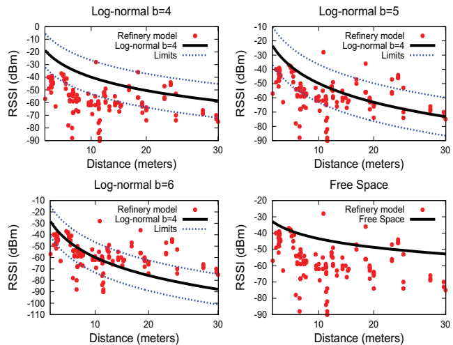
Figure 4: Comparison with theoretical values of free-space and fading models
