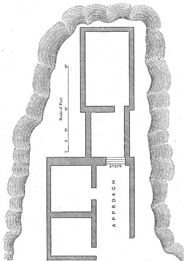
PLAN OF THE FORTRESS AT APHENDRIKA.
