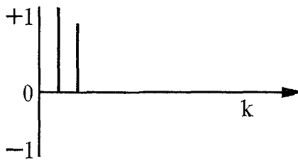
Autocorrelation function of an MA(2) model (two autocorrelations significantly different from zero).
