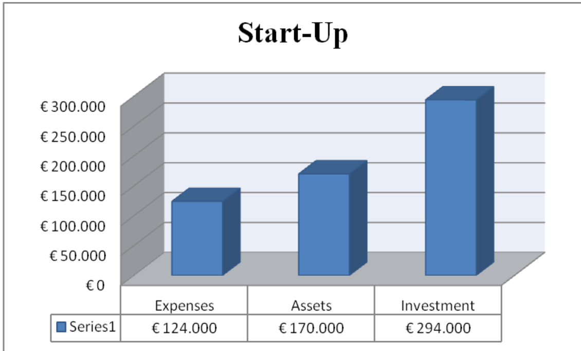
Graph 3.1: Start-up expenses, assets and investment
