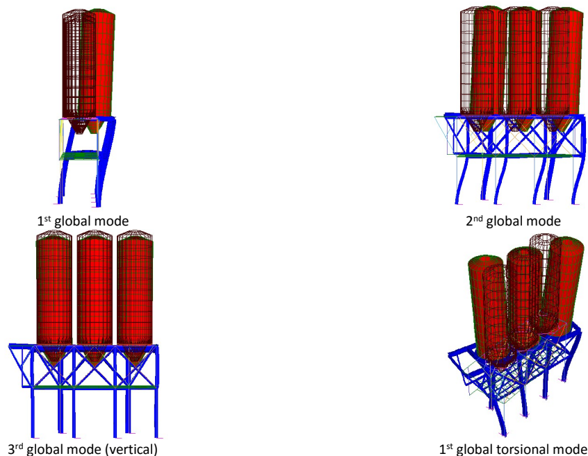
Figure 8 Mode shapes
