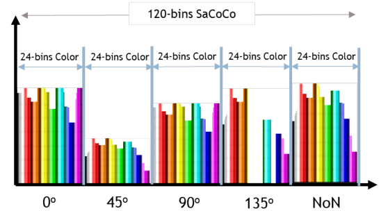
Fig. 7. The Saliency and Color Information Descriptor.
