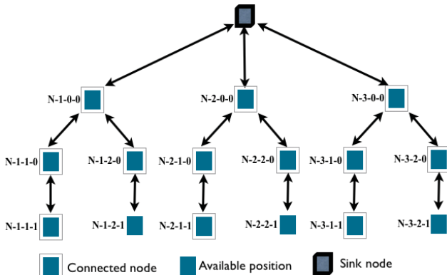
Figure 3: Tree Topology
