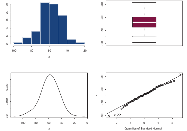
Figure 5: Histogram, boxplot, density and quantile-quantile plot of the data
