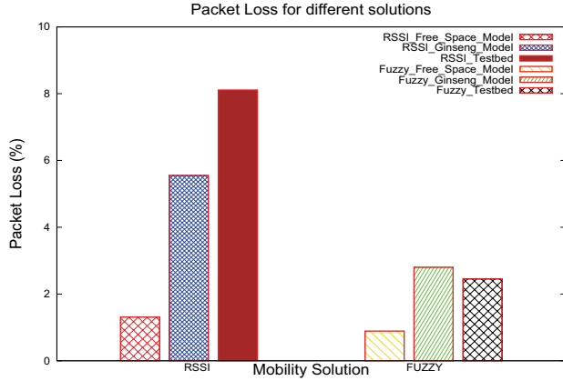
Figure 12: Reliability comparison
