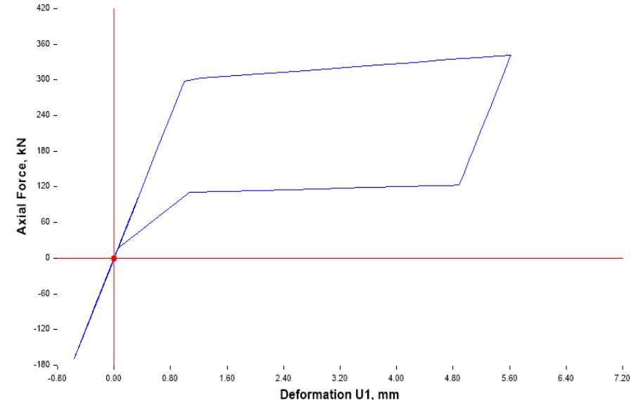
X-X-1: K14 Damper Hysteresis of ED6349 with scale factor 3.00
