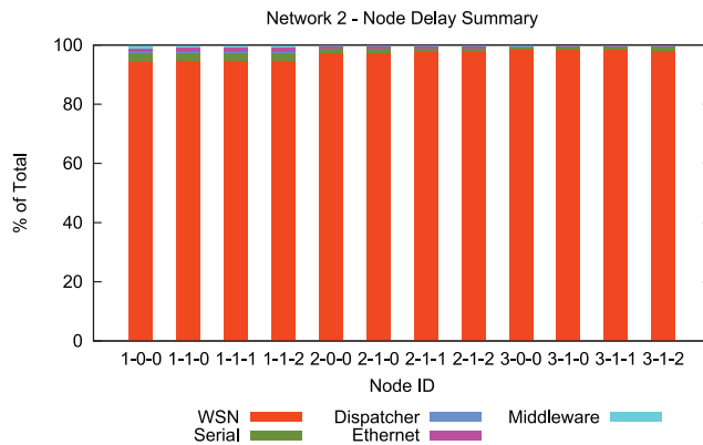
(c) Node delivery delay percentage.
