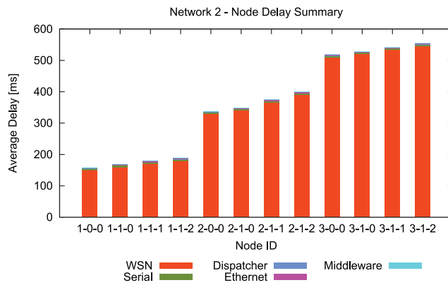
(b) Node delivery delay.
