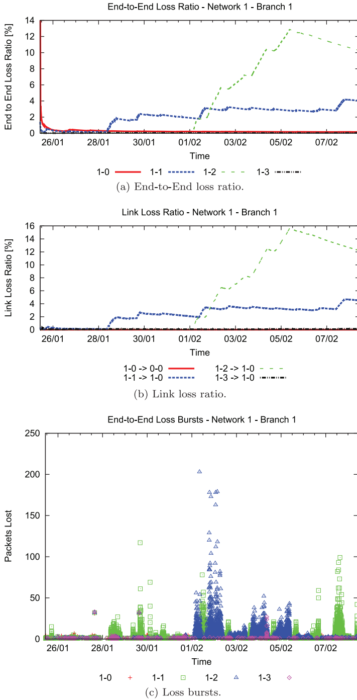
Fig. 19. Network 1, Branch 1, showing problematic links.
