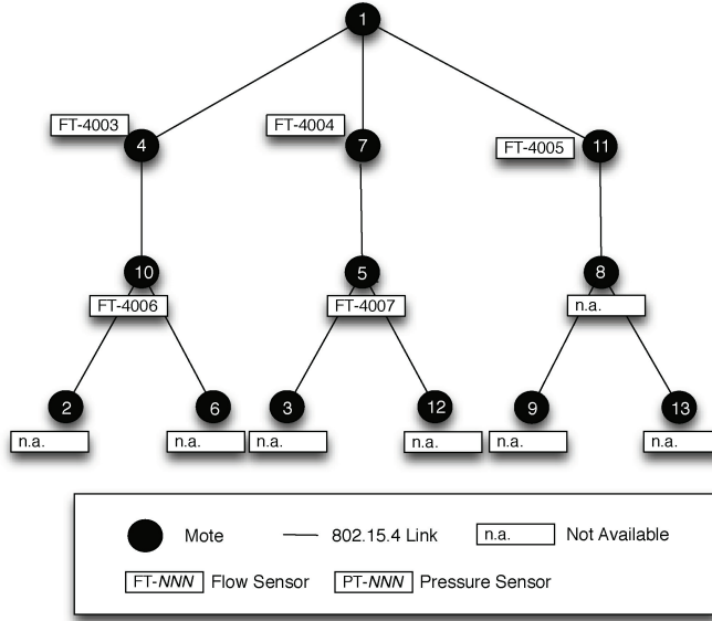
Fig. 11. Logical topology of network 2.
