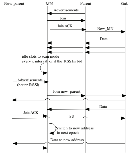
Fig. 5. Soft Handoff procedure.
