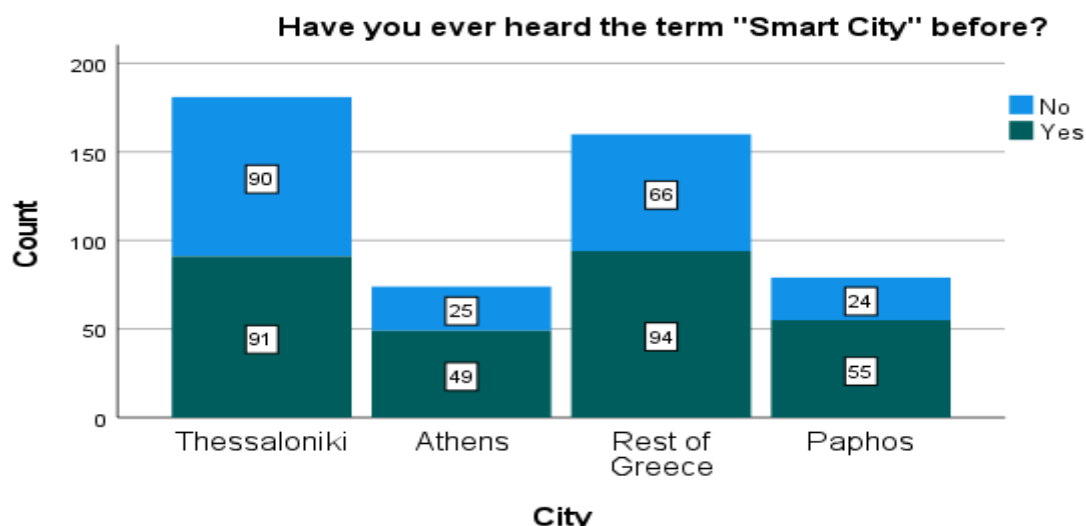
Figure 32: Results of the crosstabulation of “city” factor and of the responses in question 6
