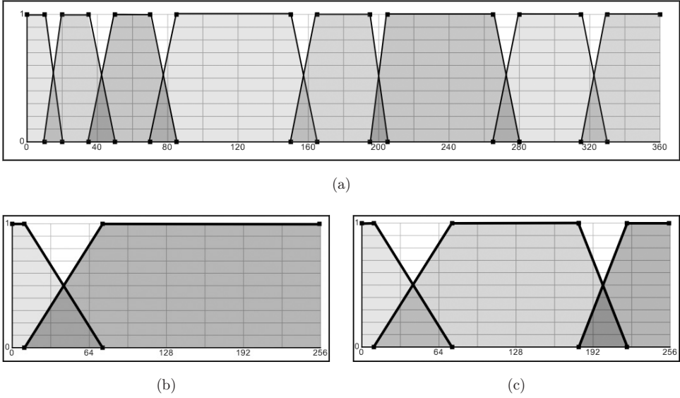
Fig. 2. Membership functions of (a) Hue, (b) Saturation and (c) Value.
