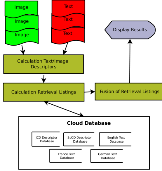
Fig. 2. System's architecture.
