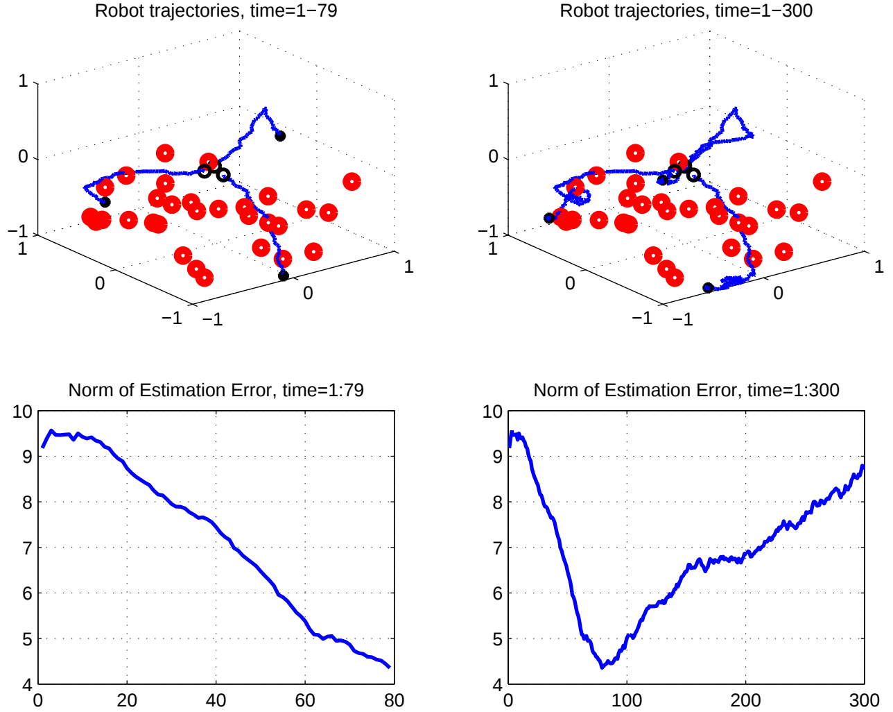
Fig. 1. Autonomous exploration by moving towards minimizing the trace of EKF error covariance matrix: N_R = 3, N_L = 30, N_T = 0 , by assuming unlimited visibility, perfect localization and infinite computing power. The estimation error starts diverging as soon as the UAVs hit the boundary of the cube [-1, +1]^3 the UAVs are constrained to remain within.
