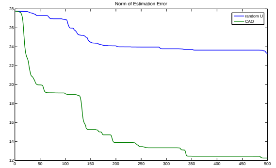
Fig. 6. Autonomous exploration using CAO and Random trajectories: N_R = 3 , N_L = 7542 , N_T = 2 . Norm of Estimation Error.
