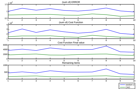
Fig. 4. Autonomous exploration using CAO and Random trajectories: N_R = 3 , N_L = 7542 , N_T = 2 . Comparison of different evaluation criteria for 10 different experiments.
