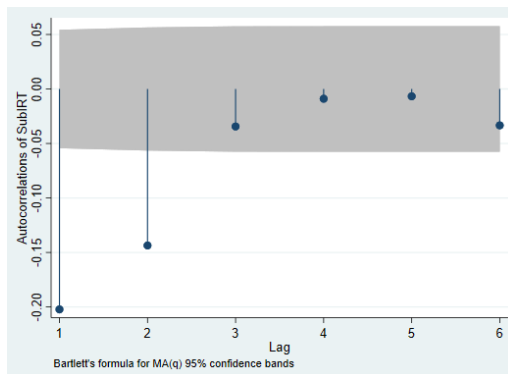
Figure 6: Correlogram NBG Sub-Period I, 2003 – 2007
