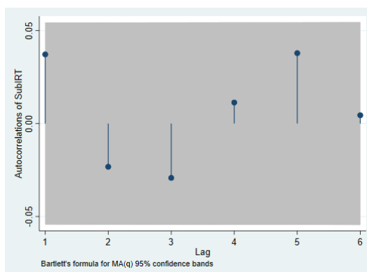
Figure 8: Correlogram Piraeus Bank Sub-Period I, 2003 – 2007
